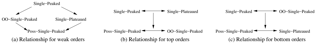
Figure 2: Relationships between the four models of single-peaked preferences for different types of votes with ties, where A \rightarrow B indicates that a preference profile satisfying model A also satisfies model B . OO-Single-Peaked and Poss-Single-Peaked refer to Single-Peaked with Outside Options and Possibly Single-Peaked respectively.
